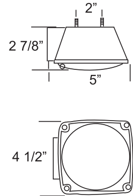
Part No. MZ-440 Turn, Tail and Stop Bolt-on
