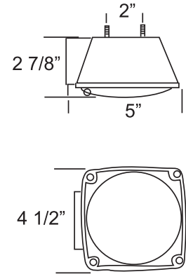
Part No. MZ-440L Turn, Tail, Stop, License Illuminator Bolt-on
