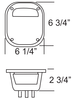
Part No. MZ-445 Turn, Tail, Stop and Backup Bolt-on
